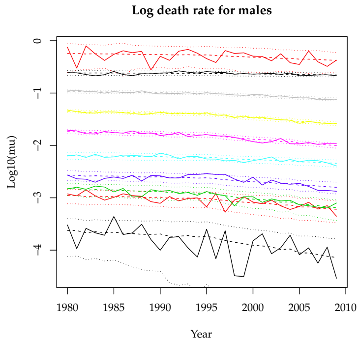
Figure 3: Data and model fit for Danish females (top) and males (bottom) for the period 1980-2009. The plots show observed death rates (solid), Lee-Carter fit (dashed) and 95% confidence intervals (dotted) for ages 10, 20, 30, 40, 50, 60, 70, 80, 90 and 100 years.
